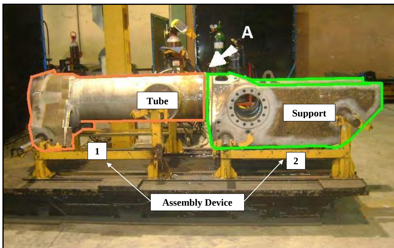
Picture 1. Frame Rear D10R
