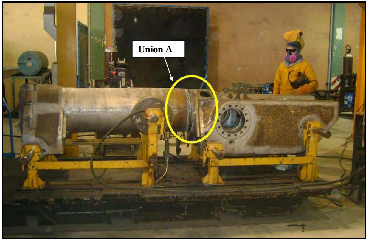
Picture 4. Welding the union “A”
